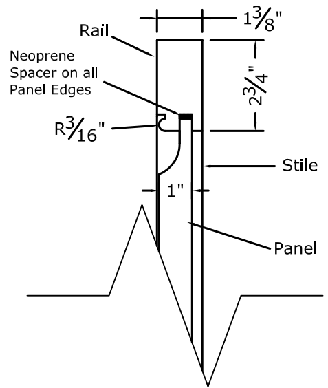
3 Panel Section
