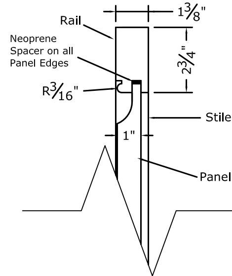
3 Panel Section
