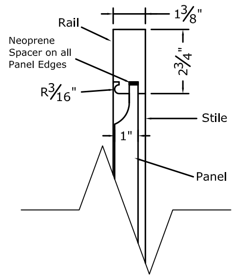
3 Panel Section
