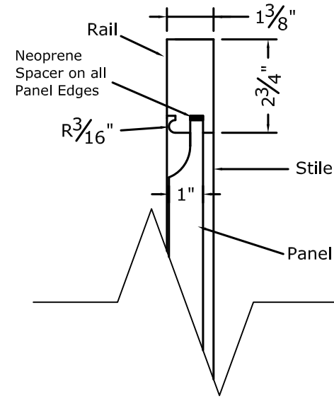
3 Panel Section
