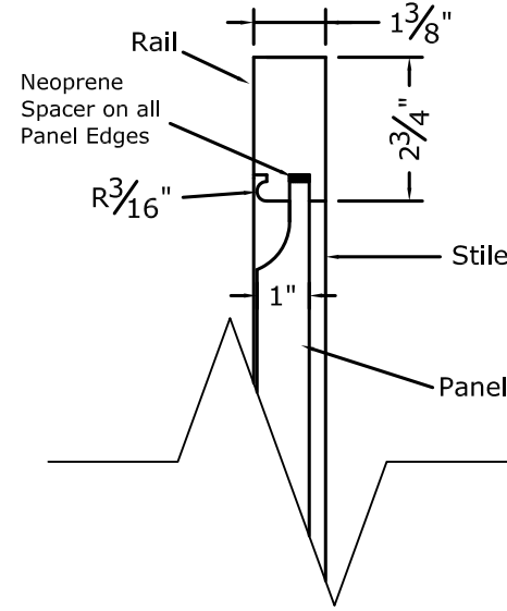
3 Panel Section
