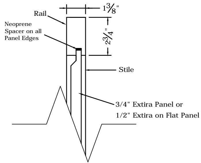
Panel Section
