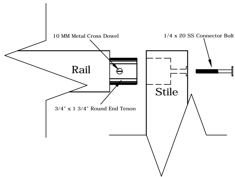
Mortise And Tenon
