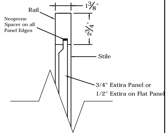
3 Panel Section
