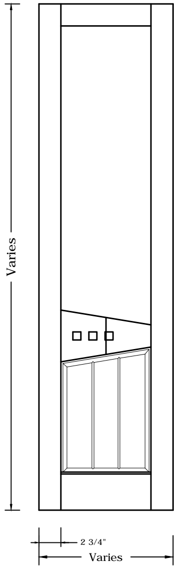
1 Front
