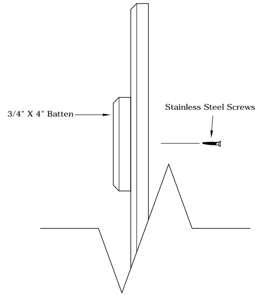
4 Batten Attachment
