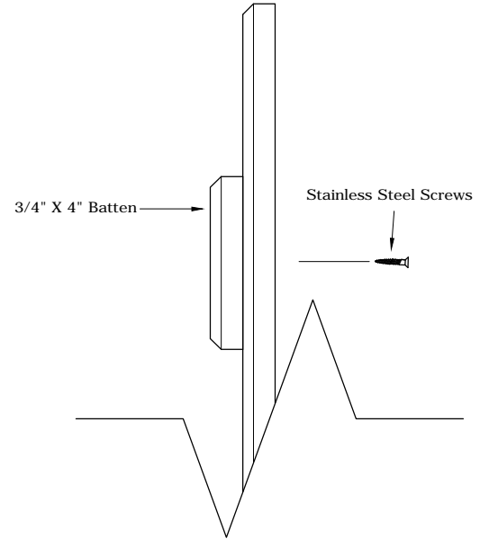
4 Batten Attachment
