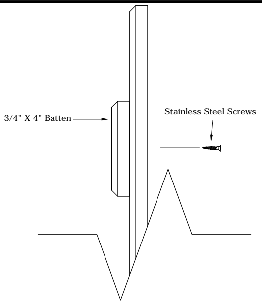
4 Batten Attachment
