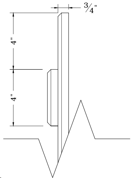
3 Panel Section
