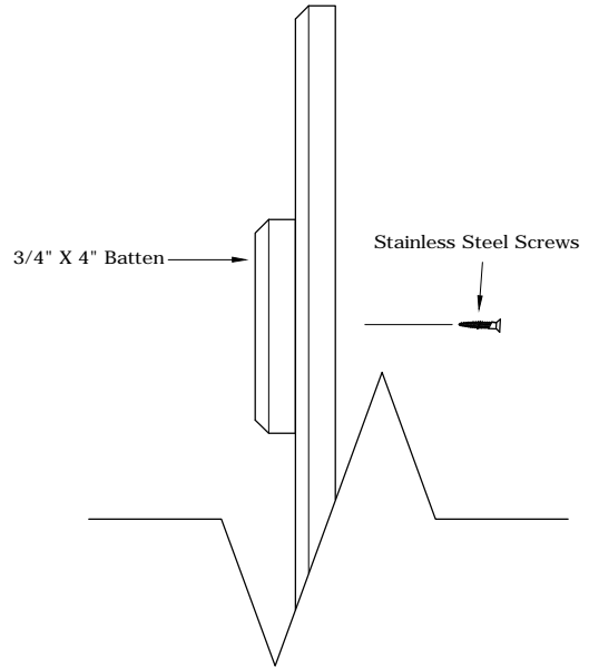
4 Batten Attachment
