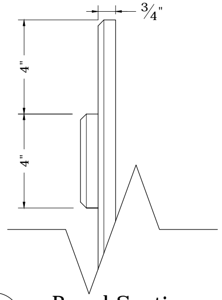
Panel Section
