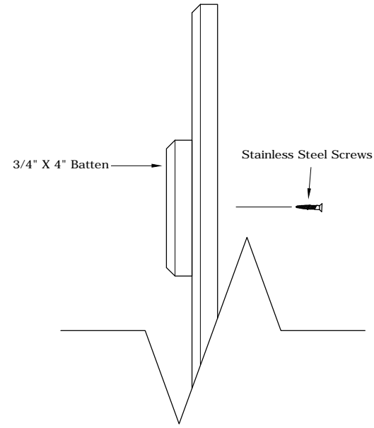
Batten Attachment
