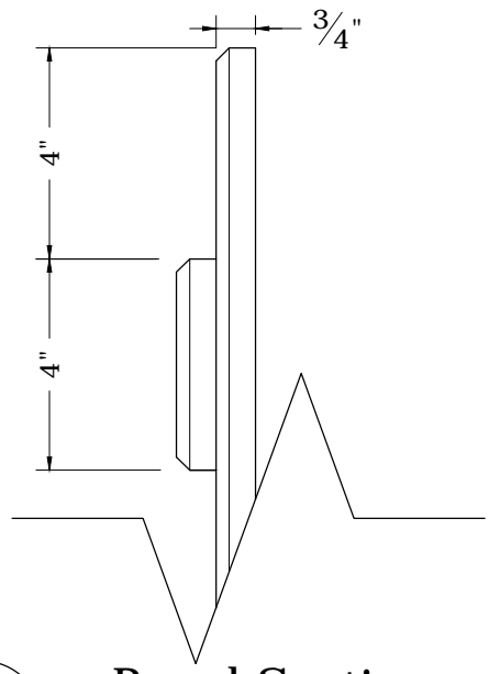
3 Panel Section
