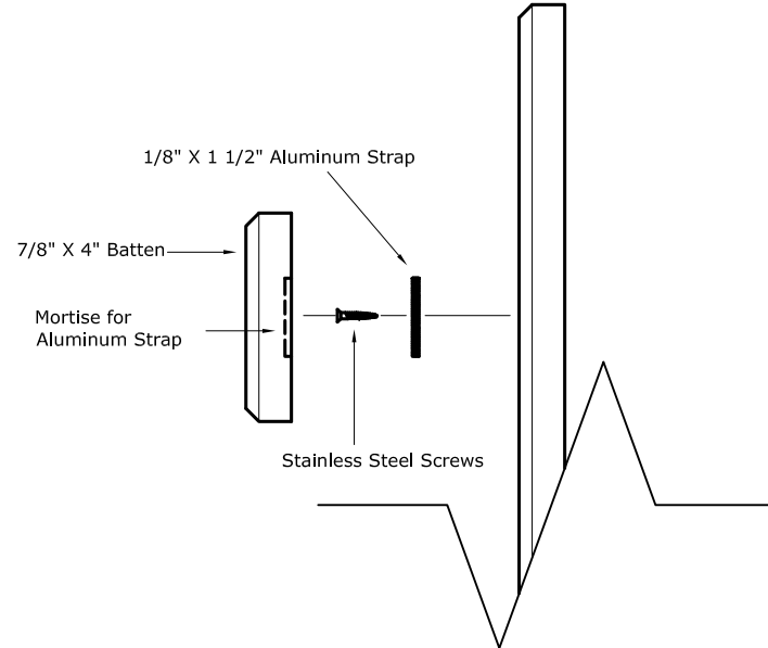
4 Batten Attachment
