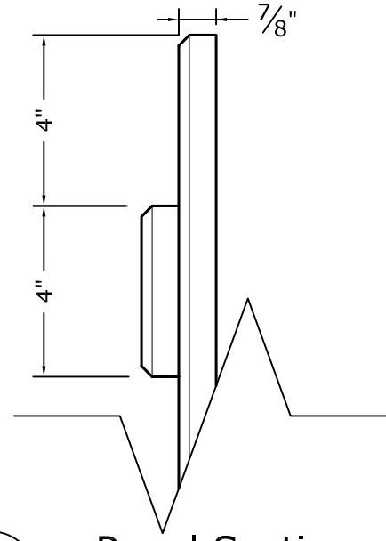
3 Panel Section
