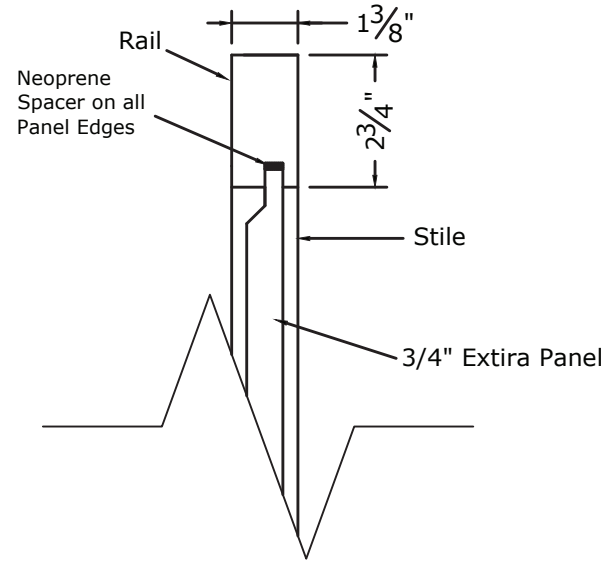
3 Panel Section
