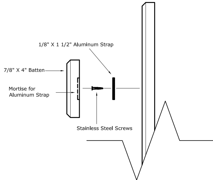
4 Batten Attachment
