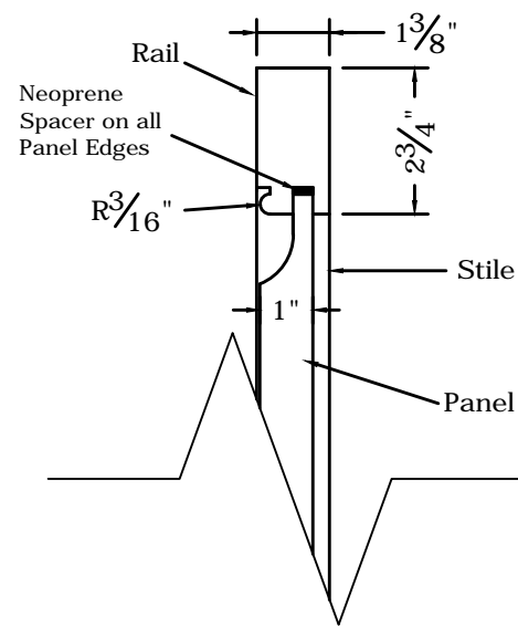
3 Panel Section
