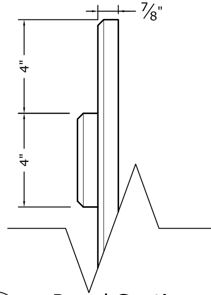
3 Panel Section
