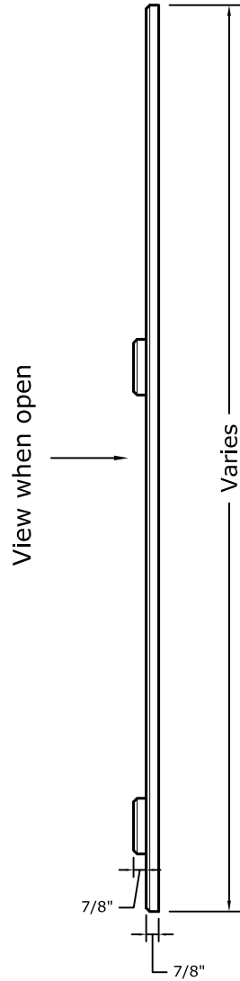
2 Side Section
