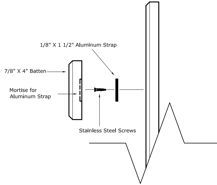
4 Batten Attachment
