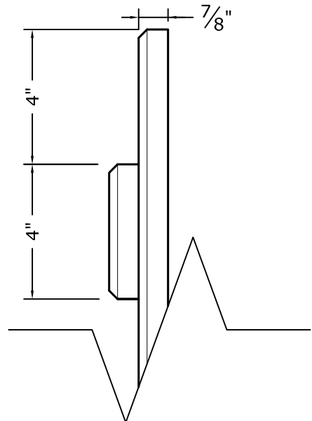
3 Panel Section
