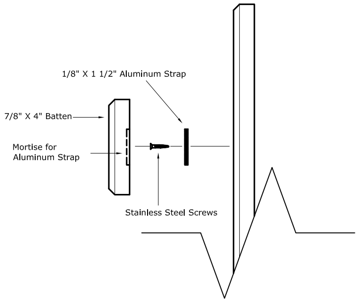
4 Batten Attachment
