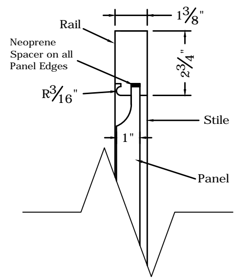
Panel Section
