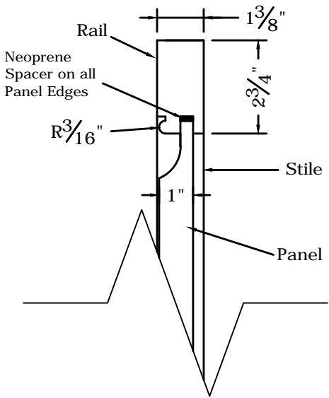
Panel Section
