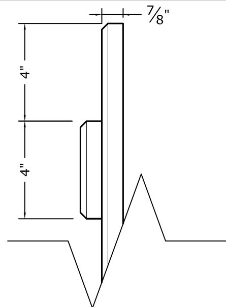
Panel Section
