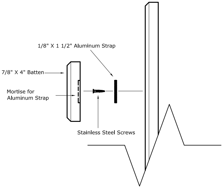
Batten Attachment
