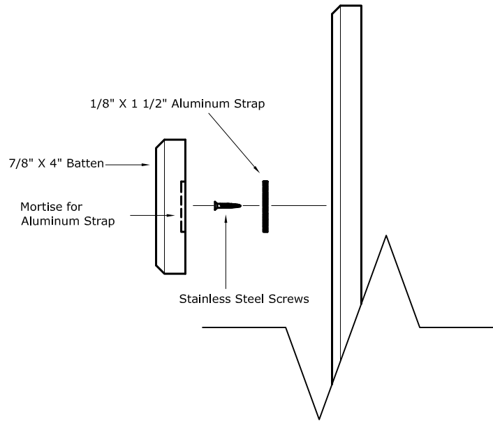
4 Batten Attachment
