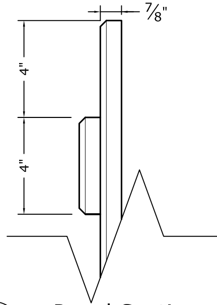
3 Panel Section
