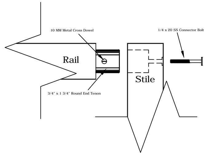
4 Mortise And Tenon
