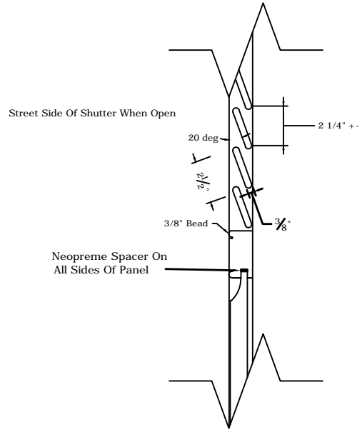
3 Panel Louver Section
