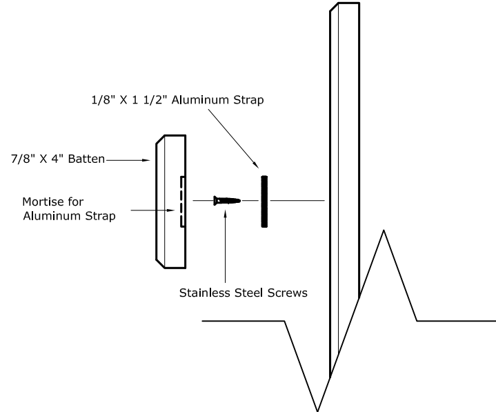
4 Batten Attachment
