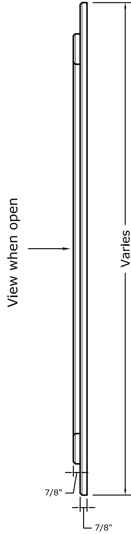
2 Stile Section
