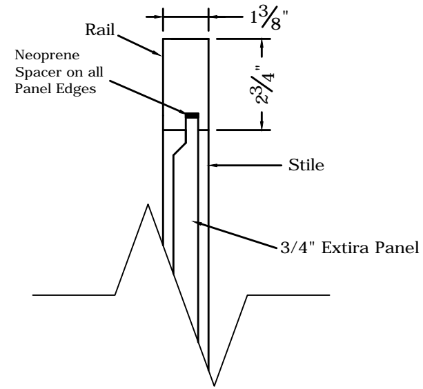
3 Panel Section
